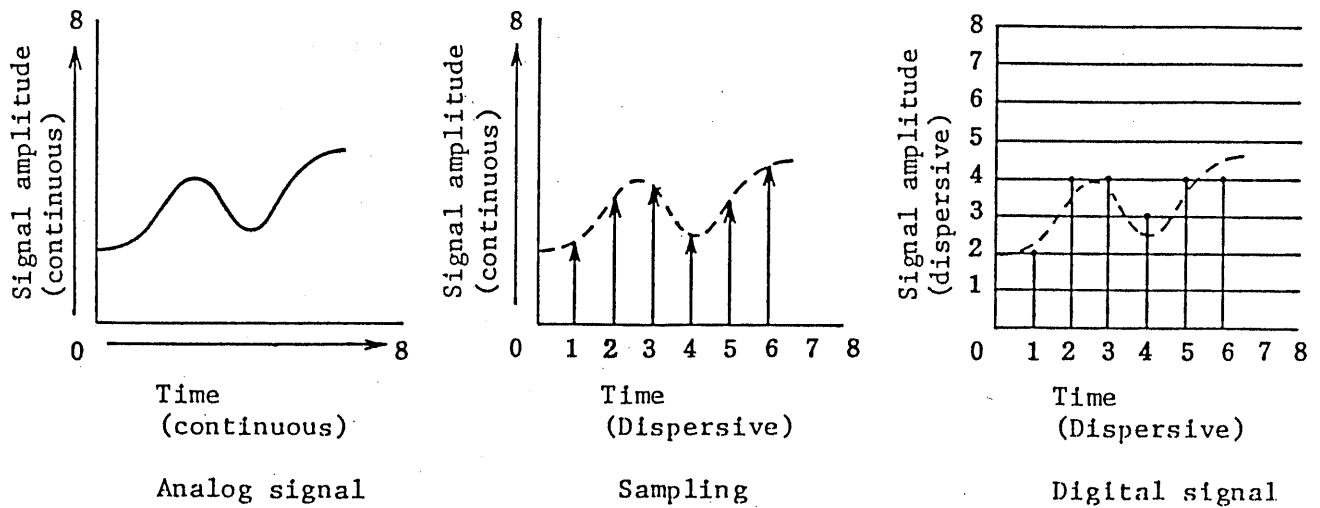
Figure 7-2. A/D Converter
