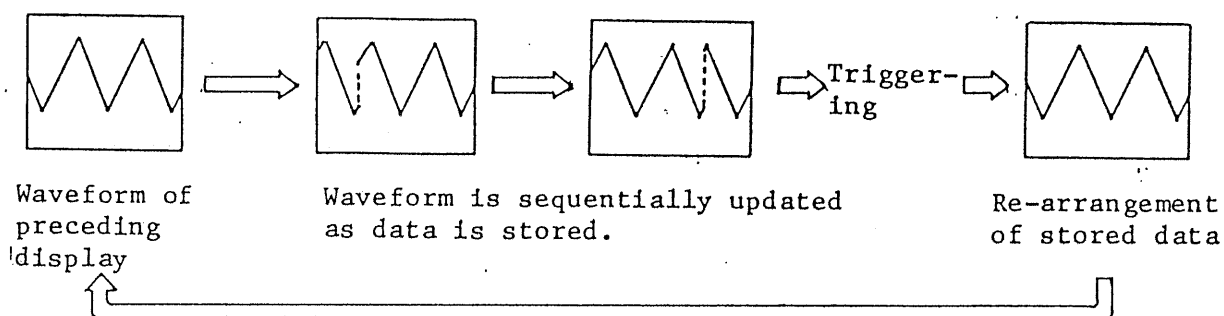
Figure 6-5. ROLL Mode
